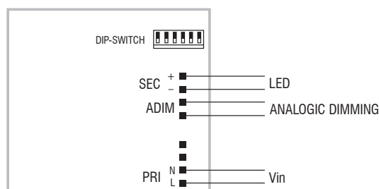
ADIM diagram - Collegamento ADIM
